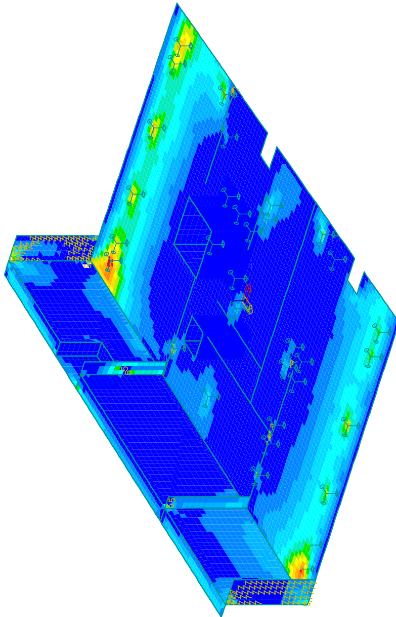
2D wapening - As1+
